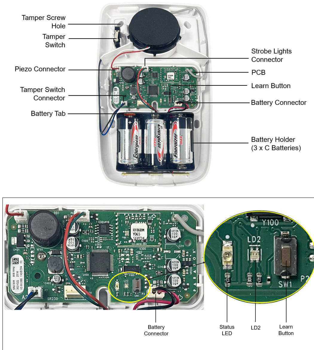
Components of SR230M
