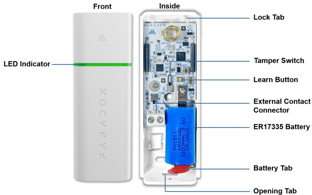
Components of DCT12M
