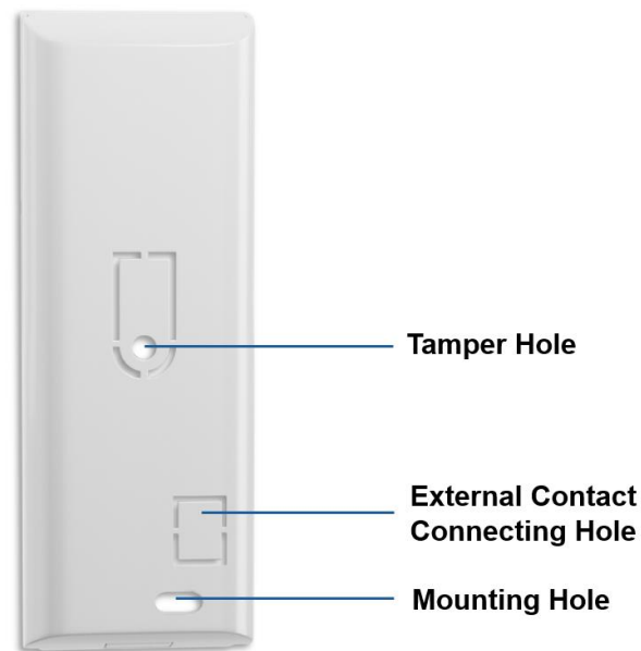
Back Side of DCT12M
