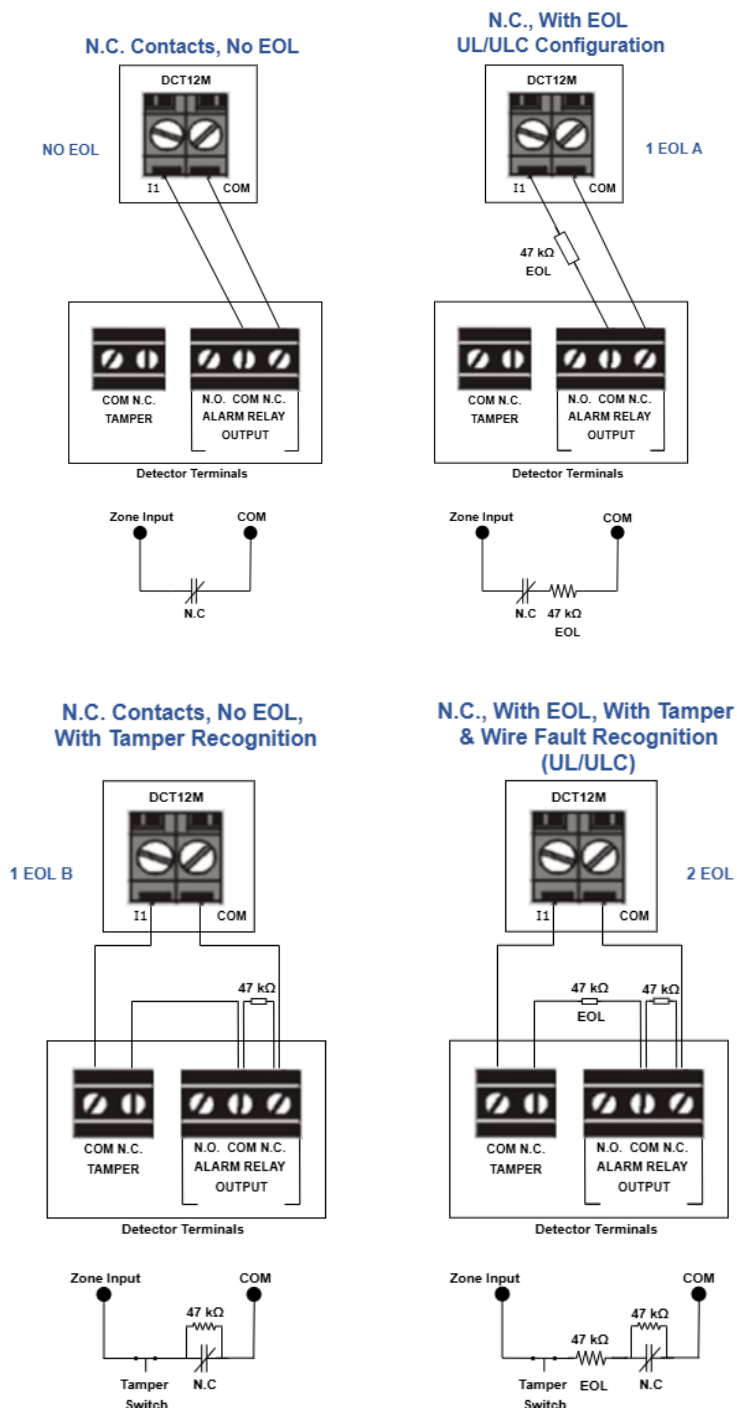
EOL Connection Options
