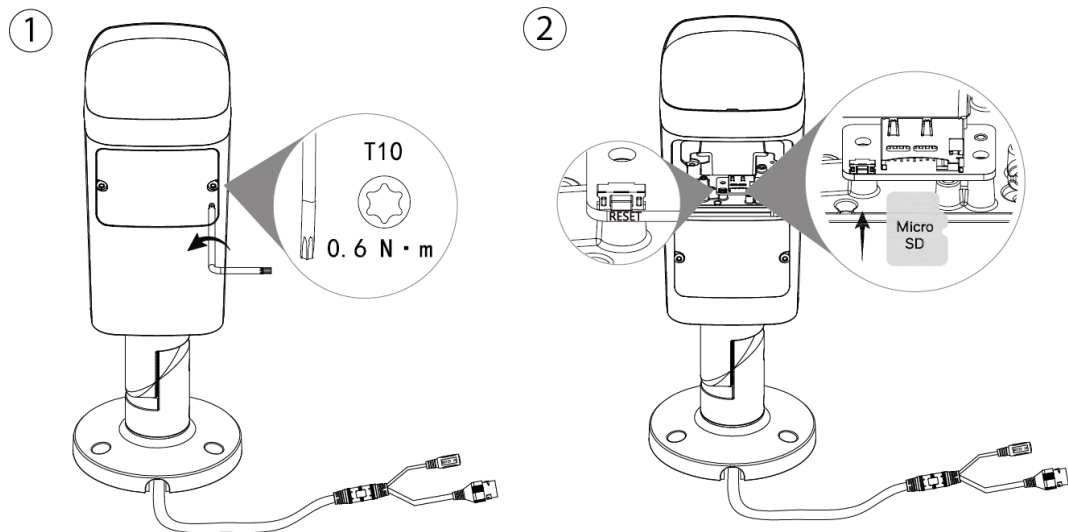
Figure 3-2 Install the SD card
