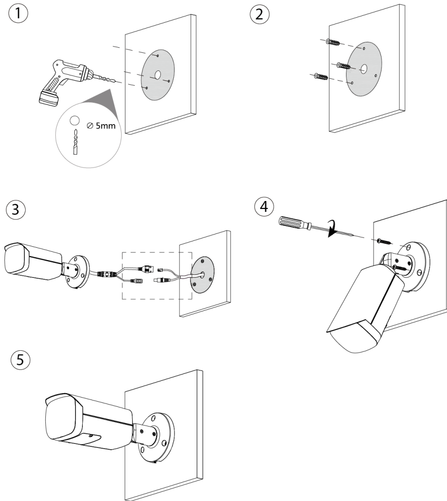
Figure 3-4 Cable going through the mounting surface
