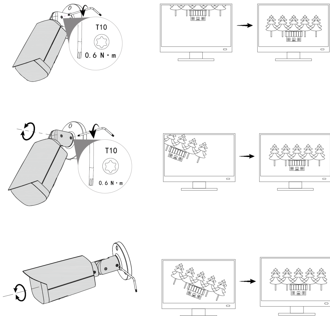
Figure 3-7 Adjust lens angle
