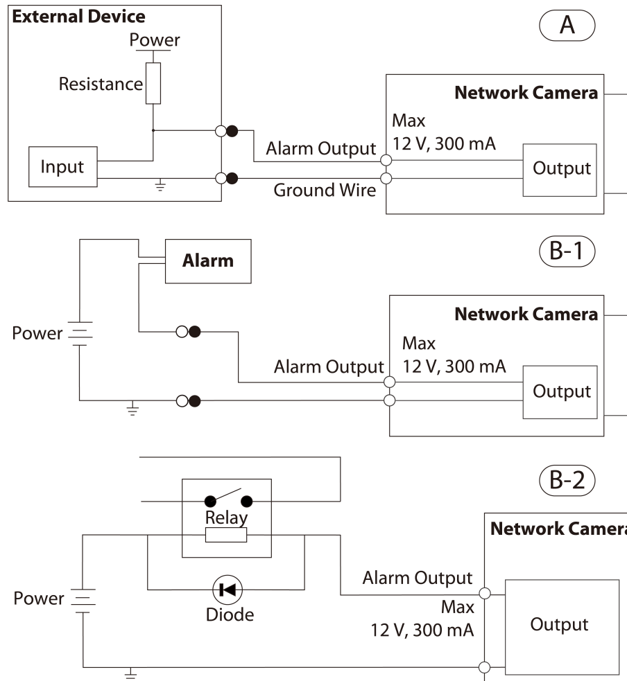
Figure 1-3 Alarm output
